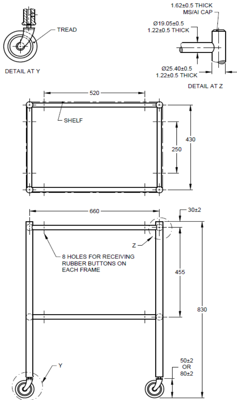
Fig. 1 PLAIN INSTRUMENT TROLLEY
